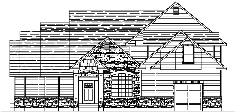
FRONT ELEVATION
