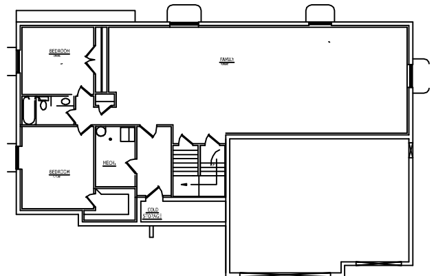
BASEMENT LAYOUT
