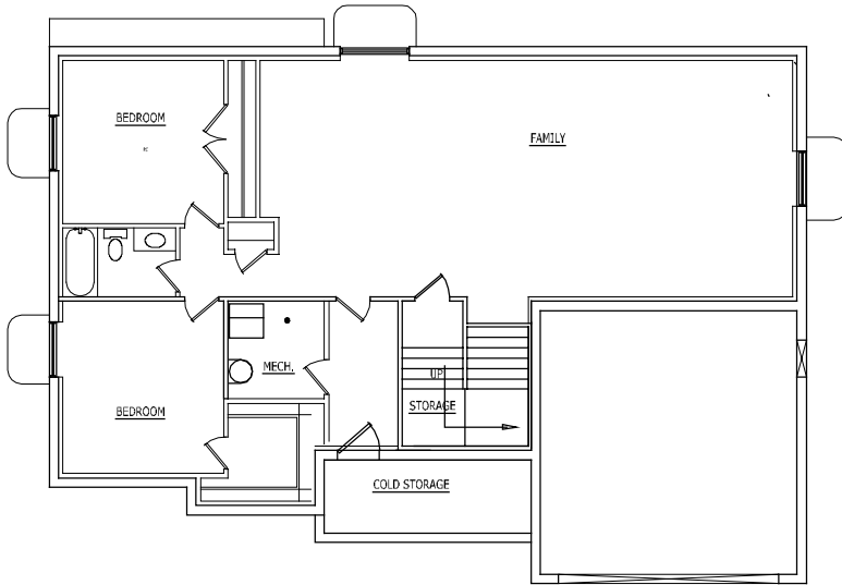
FOUNDATION PLAN SCALE 1/4" = 1'-0" 11'-0" 55'-0"
