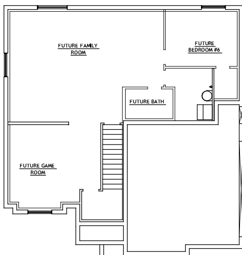
BASEMENT LAYOUT
