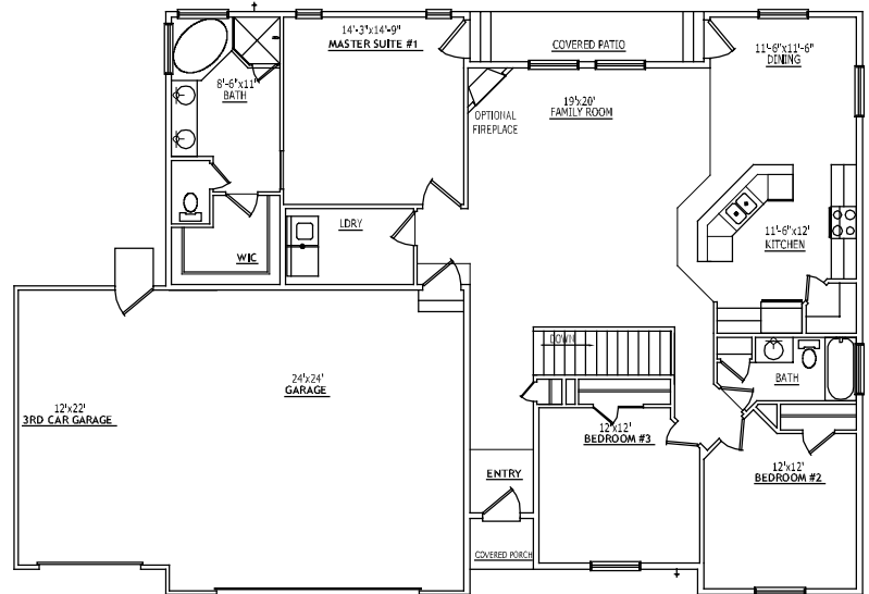
MAIN FLOOR LAYOUT
